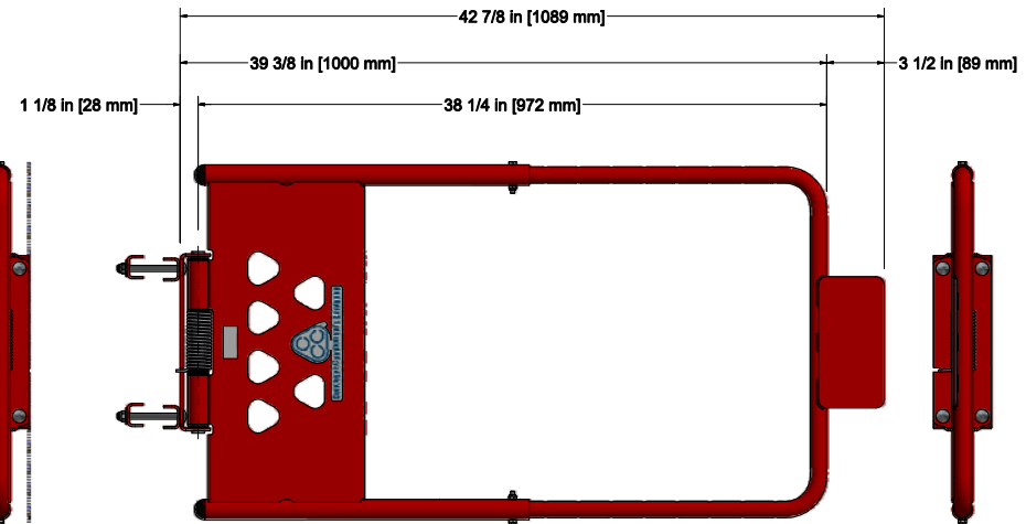
MODEL RGC-40-ZC15 SHOWN (CONVEYOR RED) 24-40" [810-1016mm] SIZE OPENING REFER TO DIMENSIONS ABOVE FOR ACTUAL SIZE
