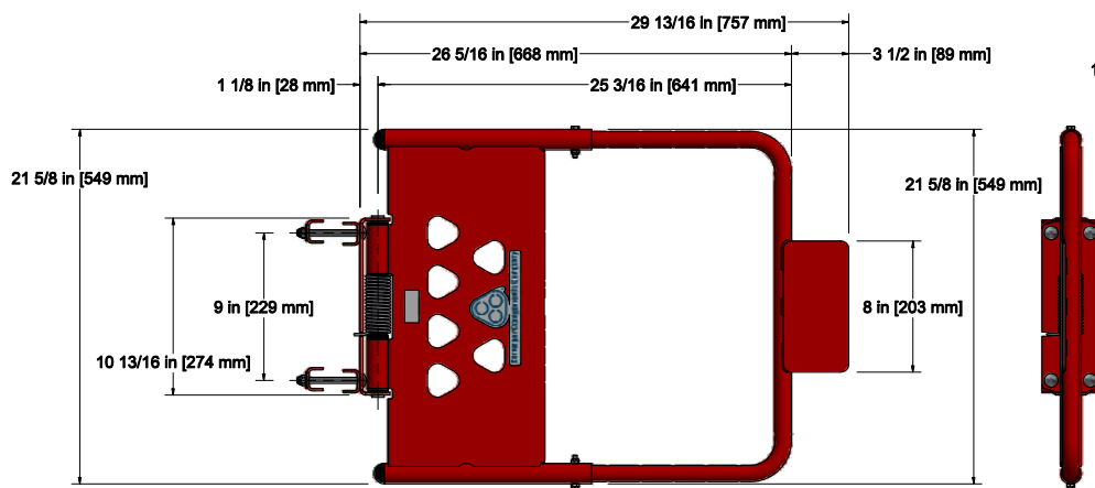
MODEL RGC-26-ZC15 SHOWN (CONVEYOR RED) 16-26" [406-660mm] SIZE OPENING REFER TO DIMENSIONS ABOVE FOR ACTUAL SIZE
